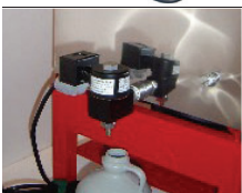
Electric bottling valve Includes 3 stainless steel tips: 1/4", 3/8", 1/2" 67217 $495.00
